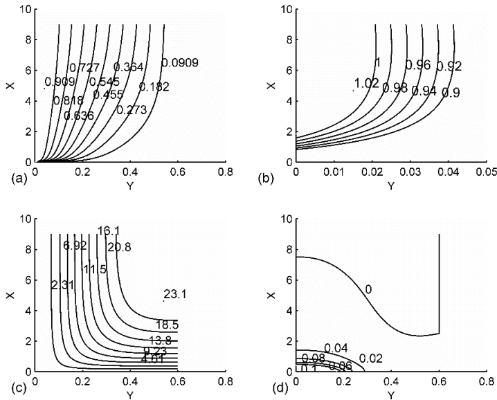
Fig. 6. The \theta (a), \phi/(1/N) (b), \Psi (c) and \partial\phi/\partial x (d) fields for Ra = 5000 , N = 5 , Le = 1 , Pr = 0.72 and S_c = 0.04 .
