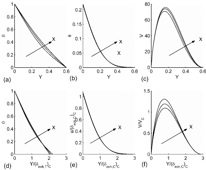
Fig. 8. The (a) \theta , (b) \phi and (c) V variations as a function of Y and the scaled (d) temperature, (e) concentration and (f) vertical velocity plots for the abscissa: 4.0, 5.0 and 6.0.
