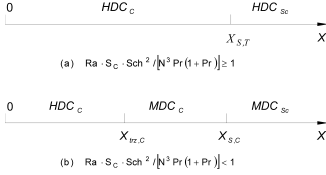
Fig. 2. The heat and mass driven natural convection regimes sequence. (a)
