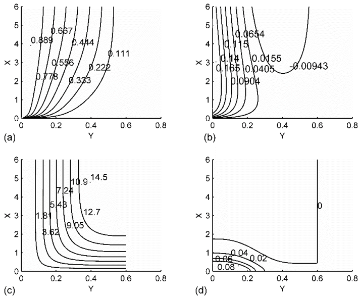
Fig. 3. The dimensionless temperature (a), concentration (b), stream function (c) and \partial \varphi / \partial x (d) fields for Ra = 5000 , N = 1 , Le = 1 , Pr = 0.72 and S_c = 0.08 .
